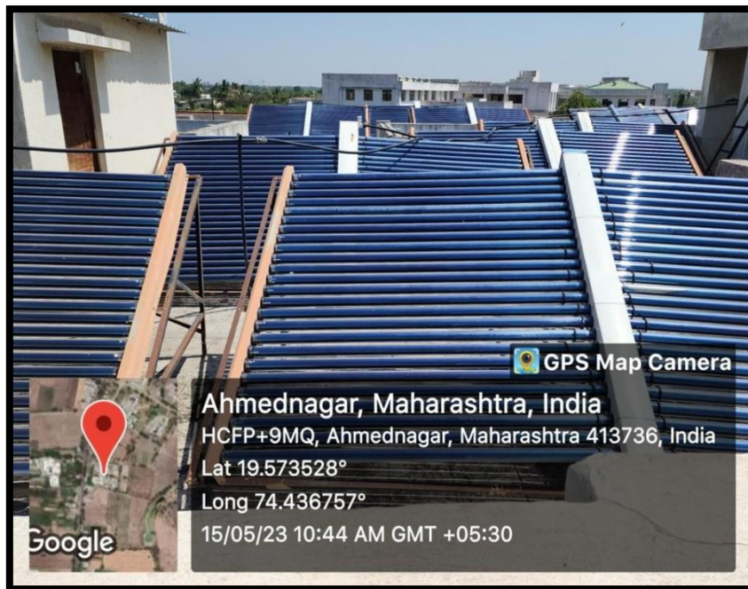
Solar Water Heater installed on Rooftop of Hostel
